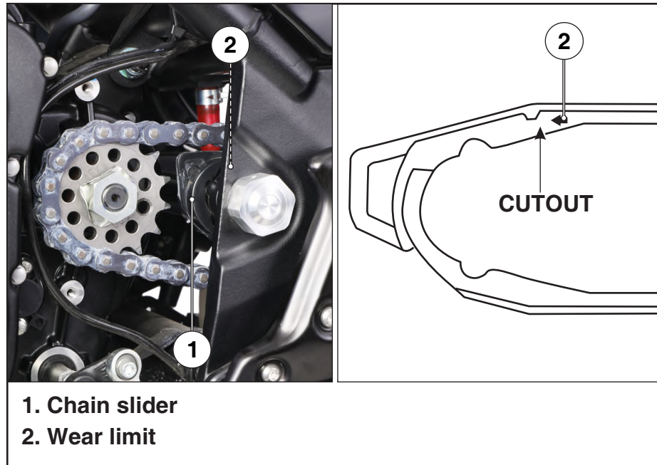
Figure 76. Drive chain slider inspection
