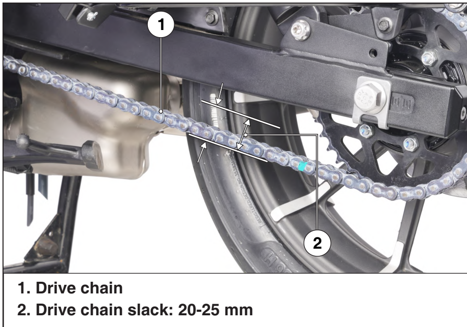
Figure 73. Drive chain slackness
