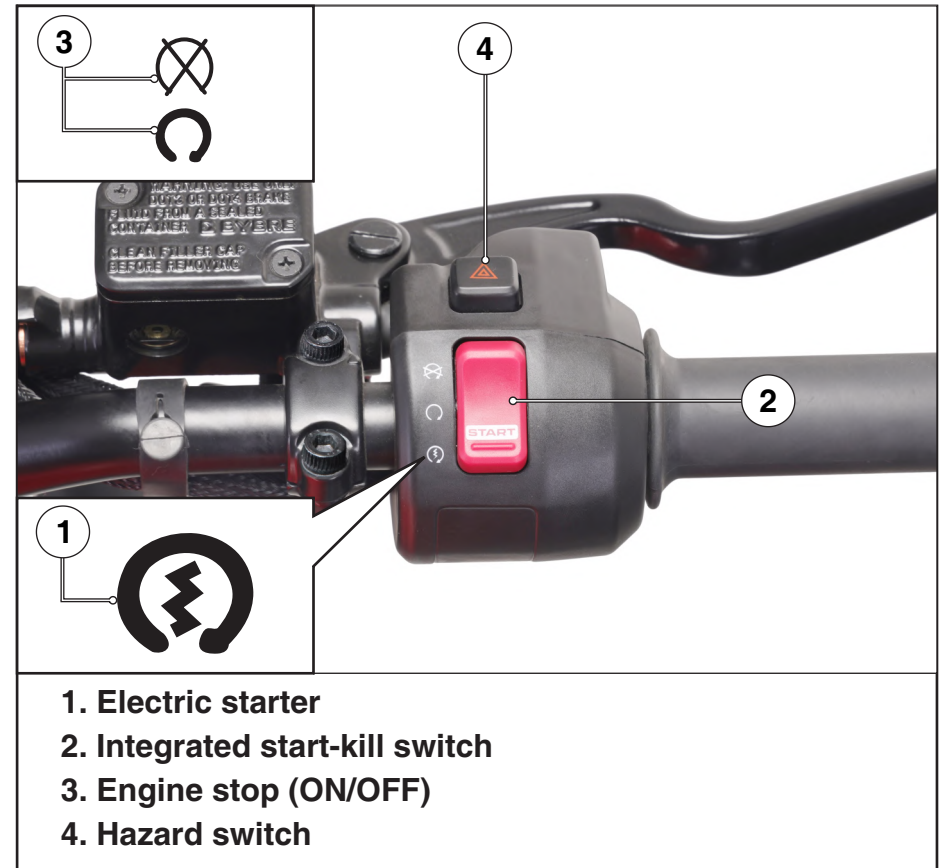
Figure 51. Right handlebar controls
