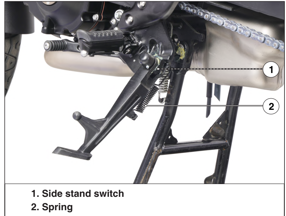
Figure 44. Side stand switch
