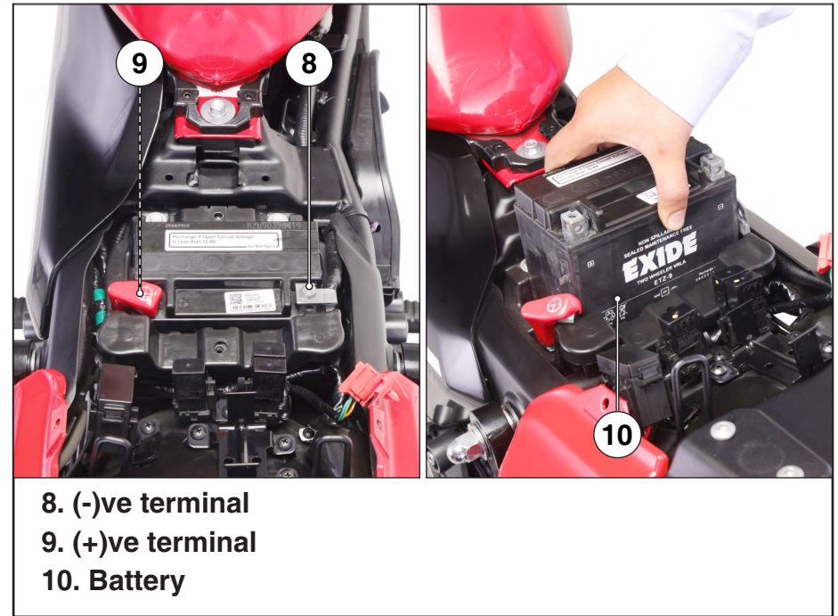
Figure 87. Battery removal
