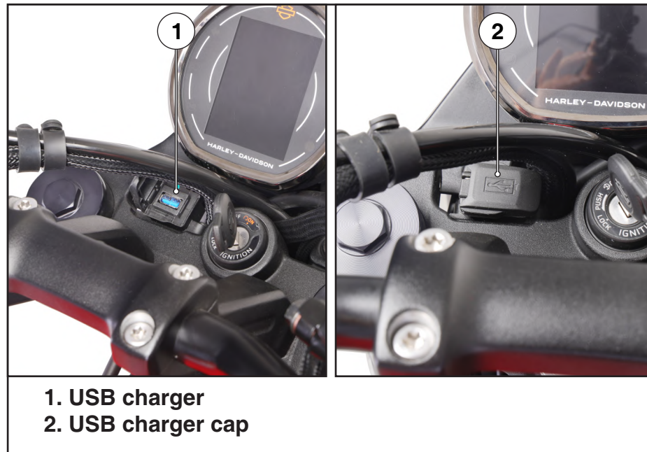
Figure 52. USB charger
