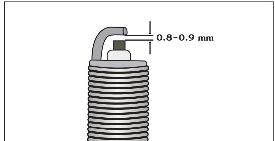
Figure 59. Spark plug
