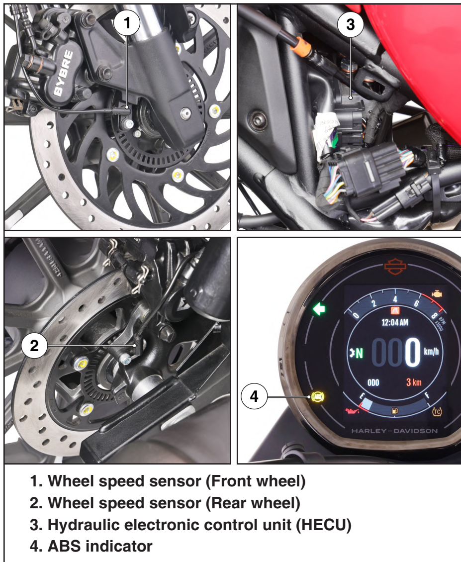
Figure 55. Anti-lock braking system (ABS)
