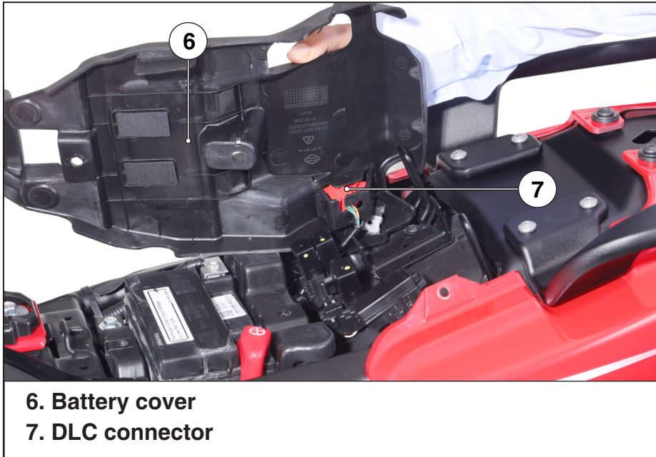
Figure 86. Battery cover removal
