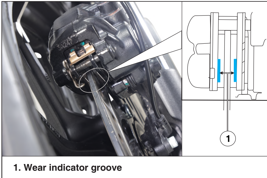
Figure 81. Front brake pad wear
