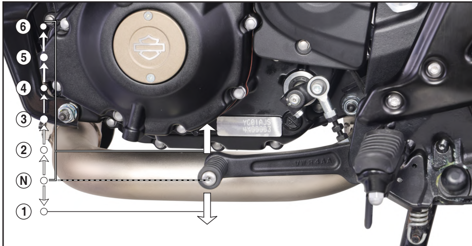
Figure 56. Gear shifting
