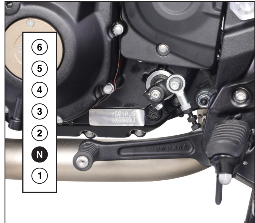
Figure 14. Shift Pattern and Shift Lever
