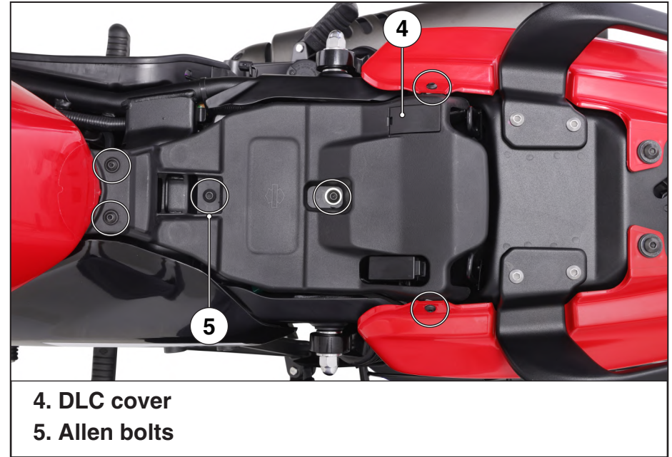
Figure 85. Battery cover removal
