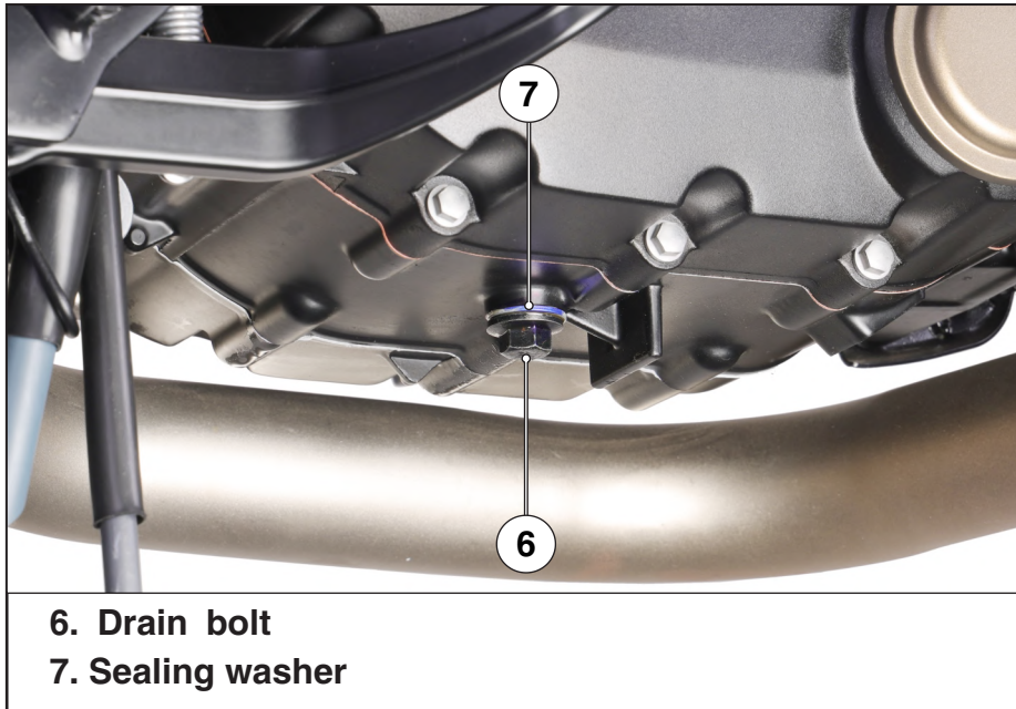
Figure 62. Engine oil replacement
