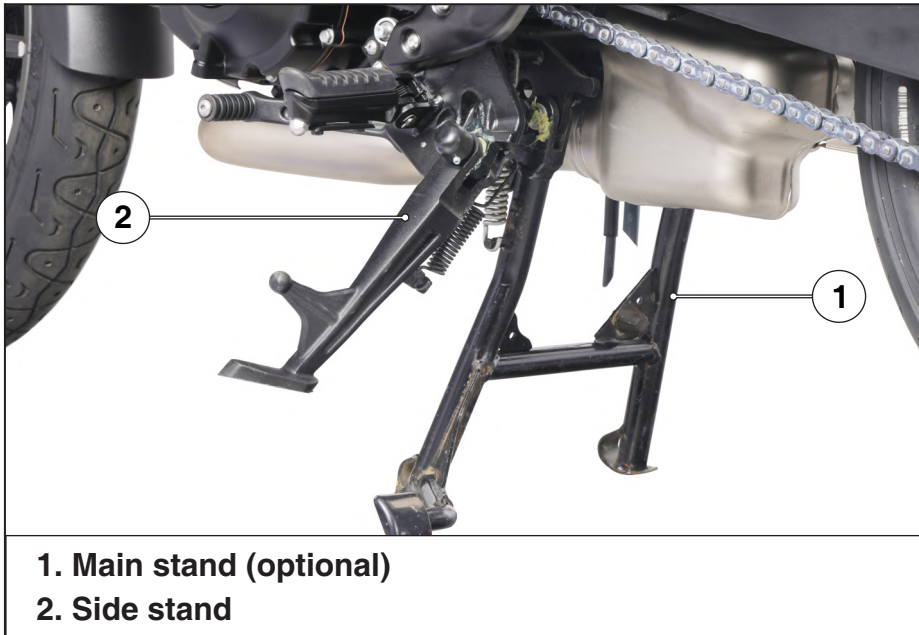
Figure 83. Main stand (optional)/Side stand
