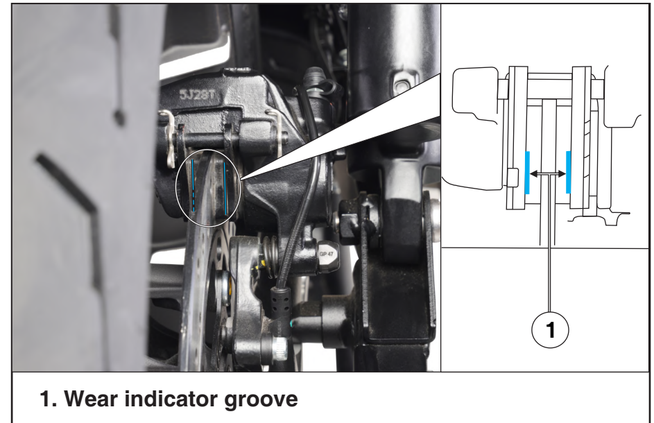
Figure 82. Rear brake pad wear
