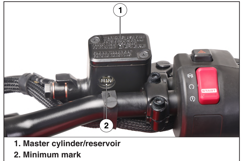
Figure 77. Master cylinder/reservoir
