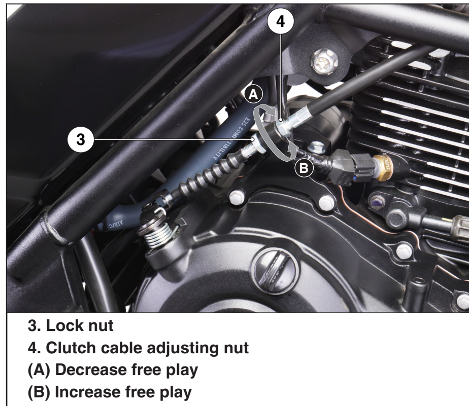
Figure 72. Clutch lever free play adjustment
