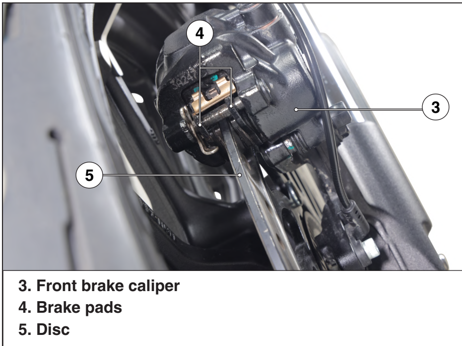
Figure 78. Front brake caliper/Pad/Disc
